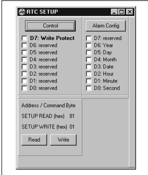
Figure 4. Setup Screen
