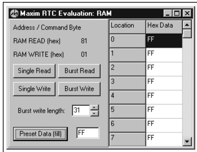
Figure 2. RAM Screen
