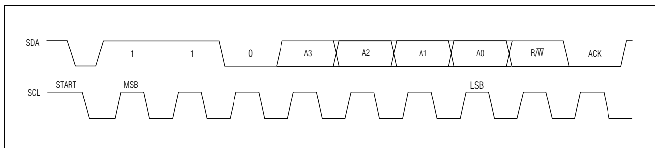
Figure 4. Slave Address
