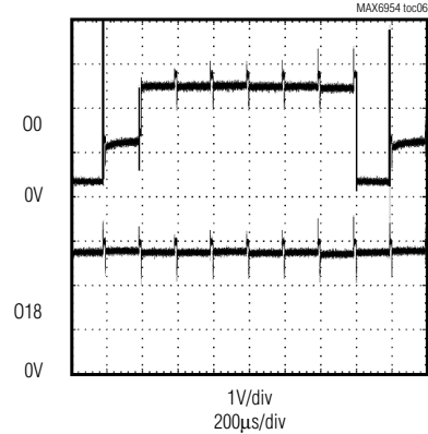
WAVEFORM AT PINS 00 AND 018, MAXIMUM INTENSITY
