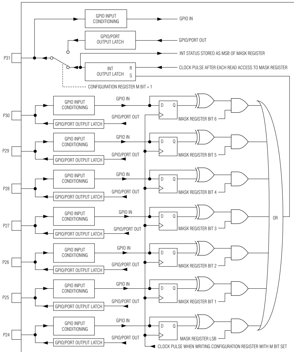
Figure 11. Maskable GPIO Ports P24 Through P31
