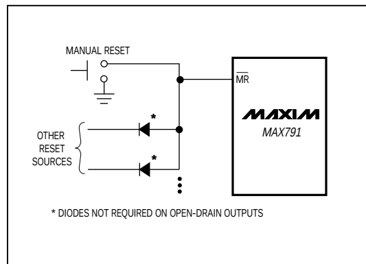
Figure 3. Diode "OR" connections allow multiple reset sources to connect to \overline{MR} .
