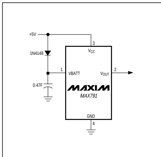
Figure 12. SuperCap or MaxCap on VBATT
