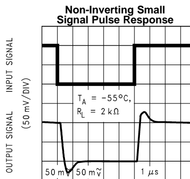
TIME (1 \mu s /DIV) Figure 42.
