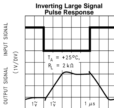
TIME (1 \mu s /DIV) Figure 44.
