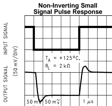
TIME (1 \mu s /DIV) Figure 40.
