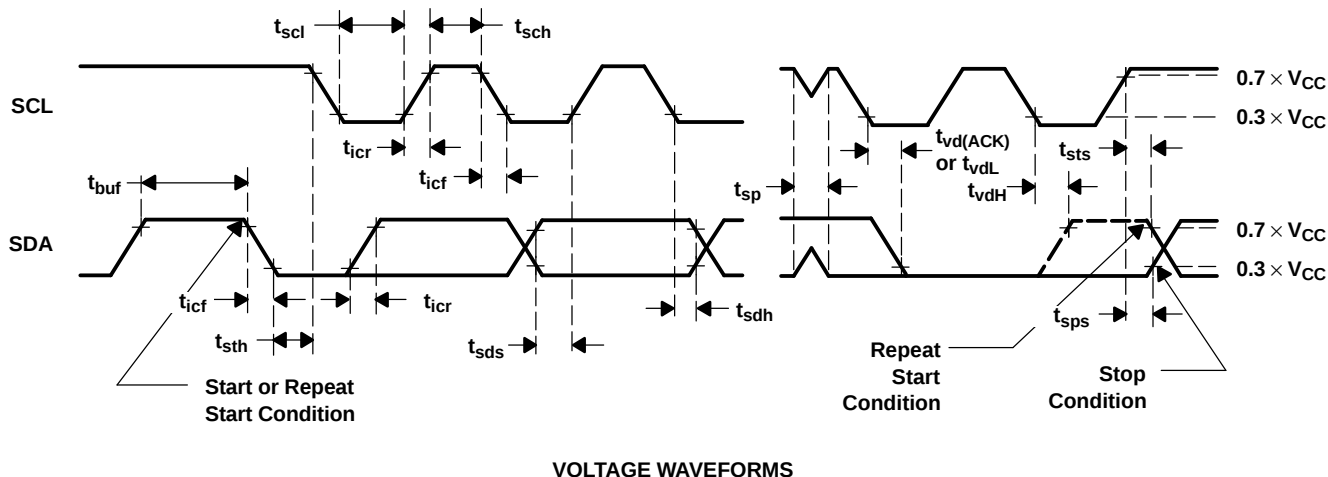
VOLTAGE WAVEFORMS
