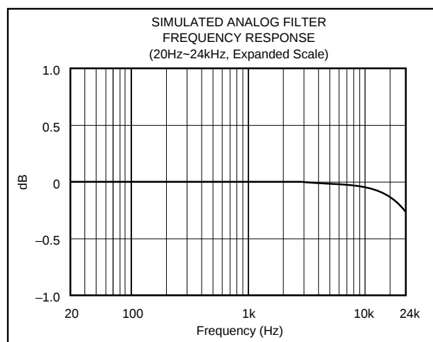
FIGURE 15. Low Pass Filter Frequency Response.
