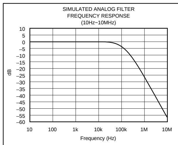
FIGURE 16. Low Pass Filter Frequency Response.
