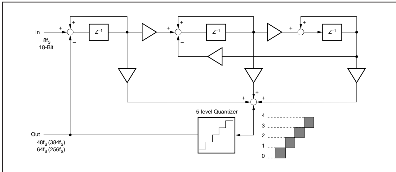
FIGURE 11. 5-Level ΔΣ Modulator Block Diagram.
