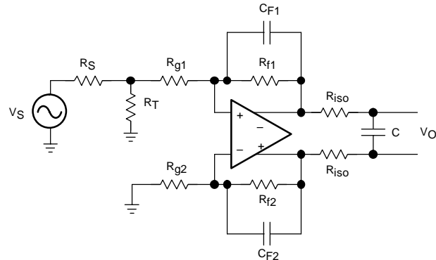
A Two-Pole, Low-Pass Filter Design Using a Fully Differential Amplifier With Poles Located at: P1 = (2\pi R_f C_f)^{-1} in Hz and P2 = (4\pi R_{iso} C)^{-1} in Hz Figure 100
