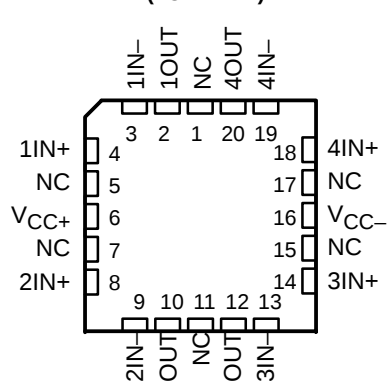
TL064 . . . FK PACKAGE (TOP VIEW)
