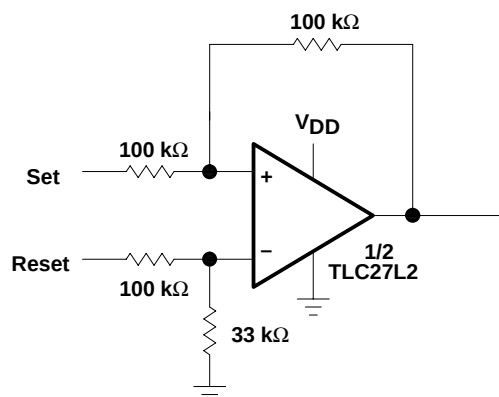
Figure 44. Multivibrator
