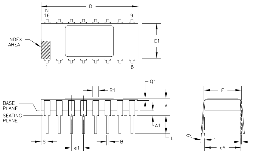
Package Number 109 - 16-Lead, Ceramic Side Braze DIP, .300 Wide
