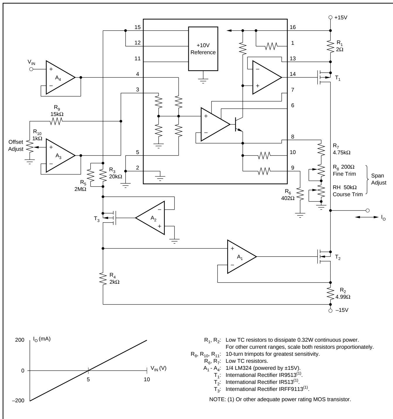
FIGURE 8. \pm 200mA Current Pump.
