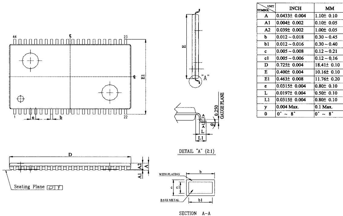
TSOP2-44
