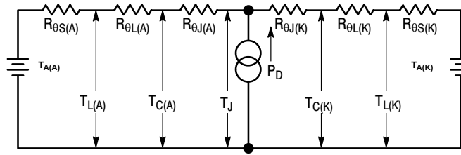
NOTE 5. — THERMAL CIRCUIT MODEL (For heat conduction through the leads)
