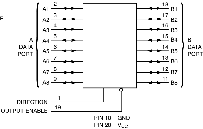
Figure 2. Logic Diagram
