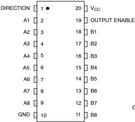
Figure 1. Pin Assignment
