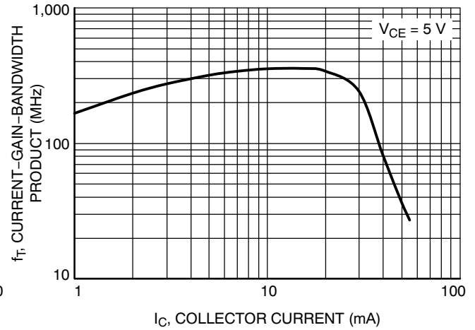
Figure 8. Current-Gain-Bandwidth Product
