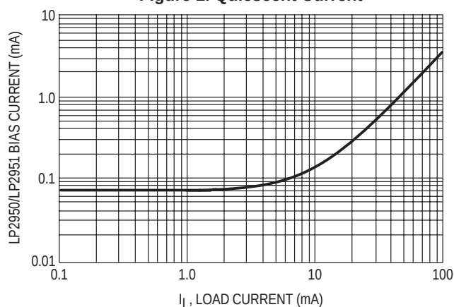
Figure 1. Quiescent Current
