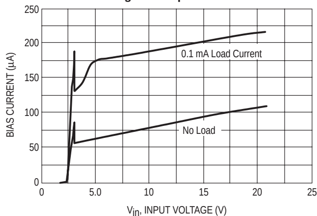
Figure 3. Input Current
