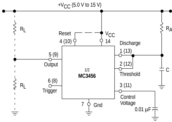
Figure 15. Monostable Circuit
