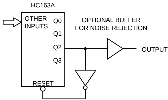
Figure 16. Modulo-5 Counter
