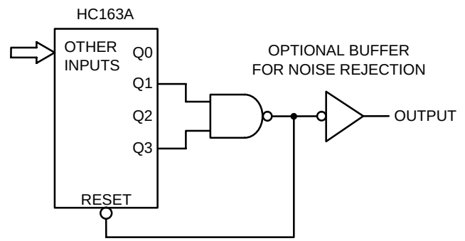
Figure 17. Modulo-11 Counter
