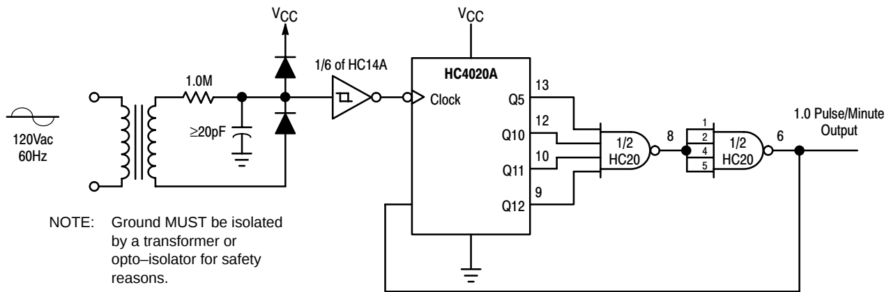
Figure 7. Time-Base Generator
