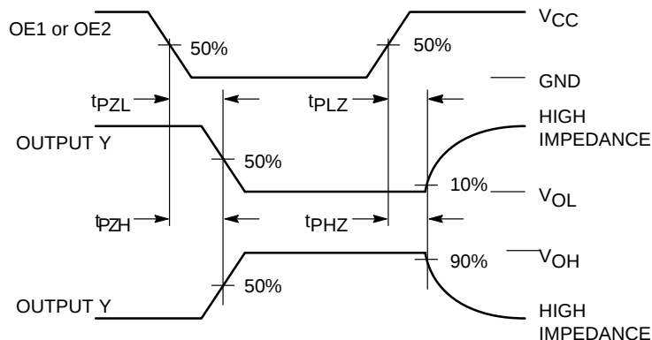
Figure 4. Switching Waveform
