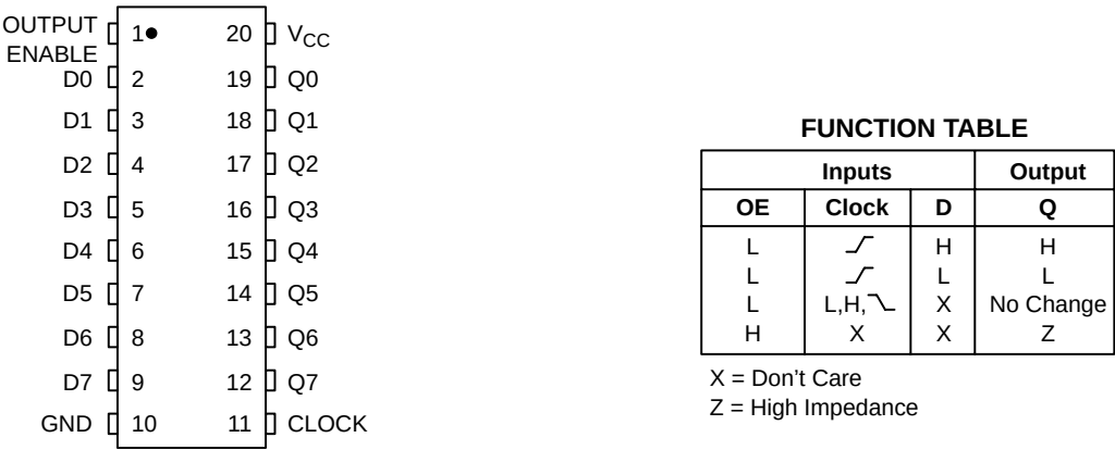
Figure 1. Pin Assignment
