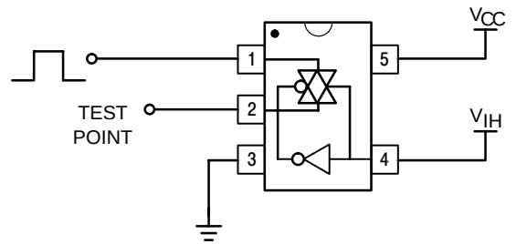
Figure 7. Propagation Delay Test Set-Up
