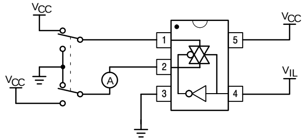
Figure 5. Maximum Off-Channel Leakage Current Test Set-Up
