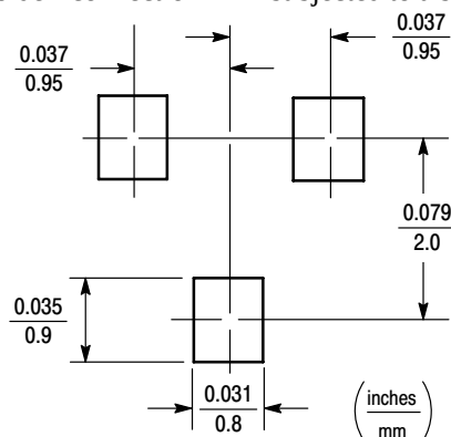
SOT-23 SOT-23 POWER DISSIPATION
