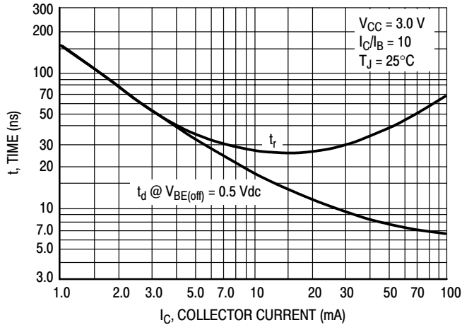
Figure 13. Turn-On Time
