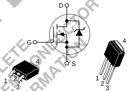
CASE 369C DPAK (Surface Mount) STYLE 2
