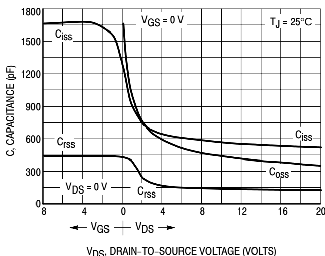
Figure 9. Capacitance Variation
