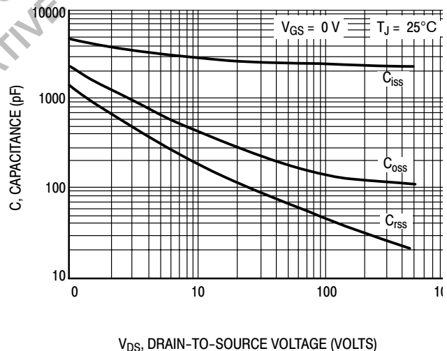
Figure 7b. High Voltage Capacitance Variation
