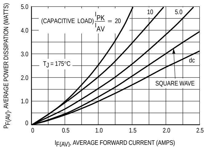
Figure 4. Power Dissipation
