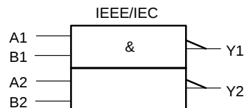
Figure 2. Logic Symbol
