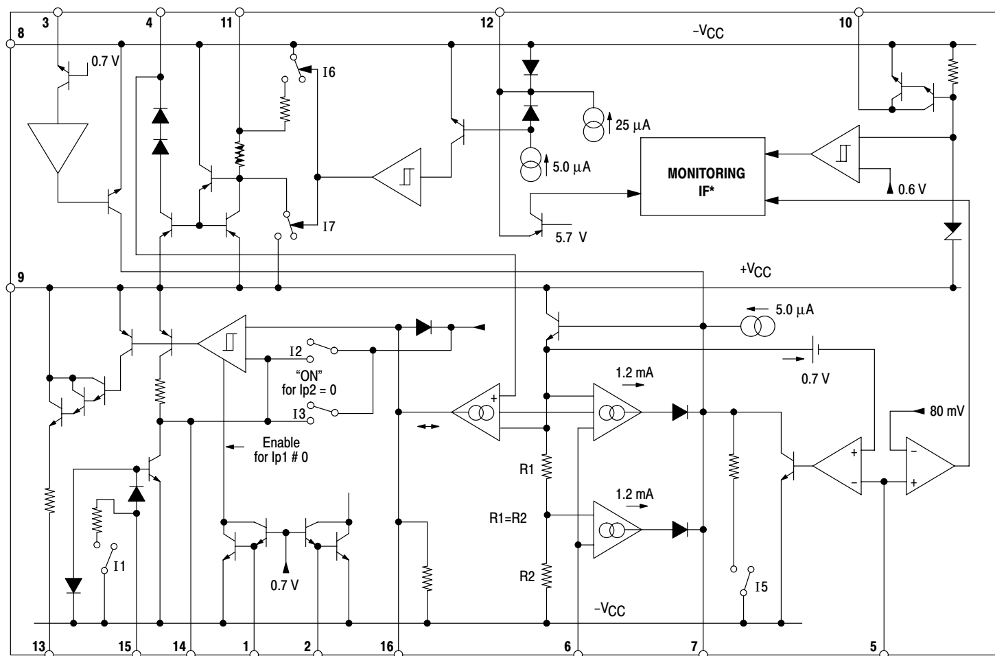
Figure 8. Simplified Schematic
