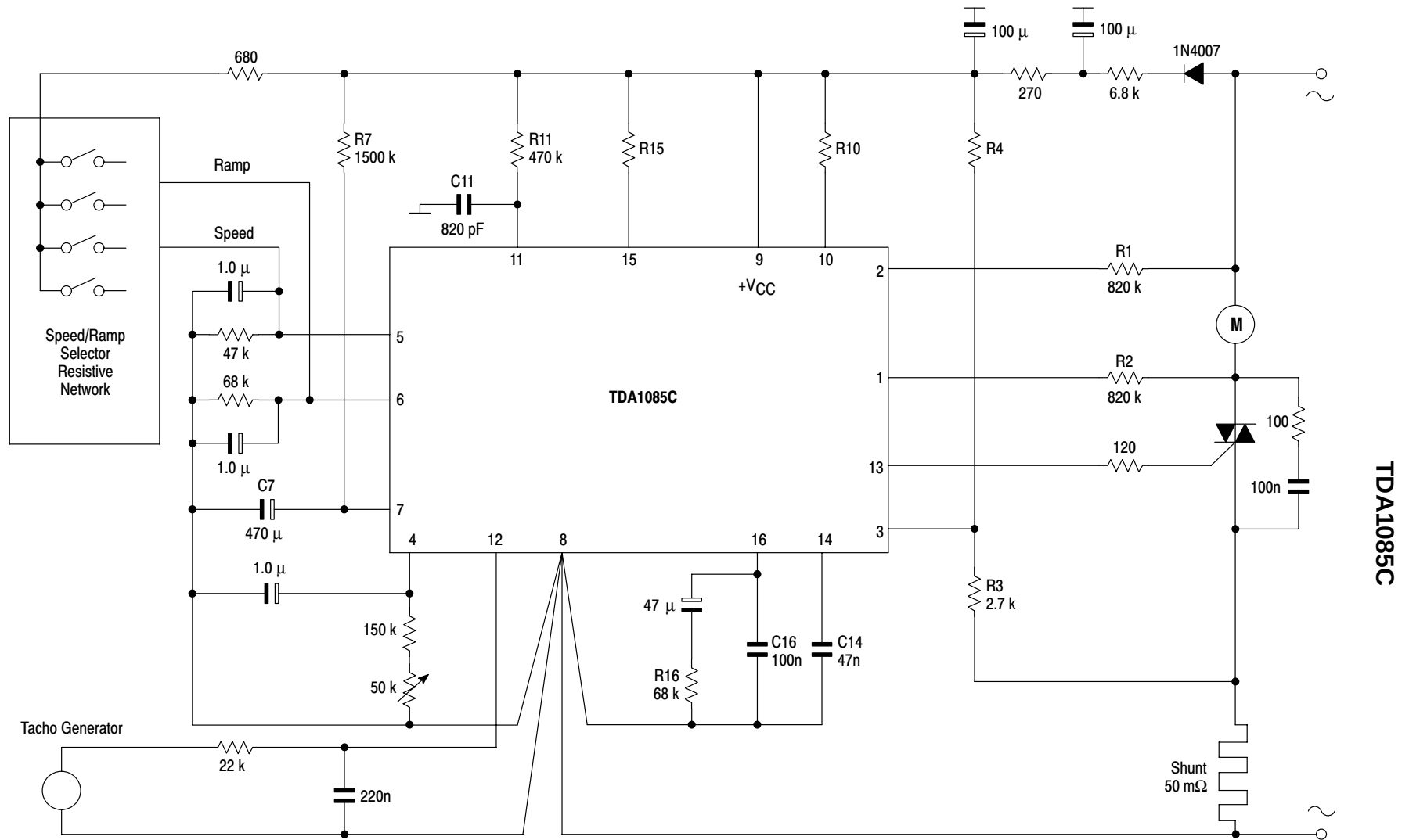
Figure 4. Basic Application Circuit
