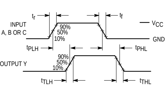
Figure 1. Switching Waveforms
