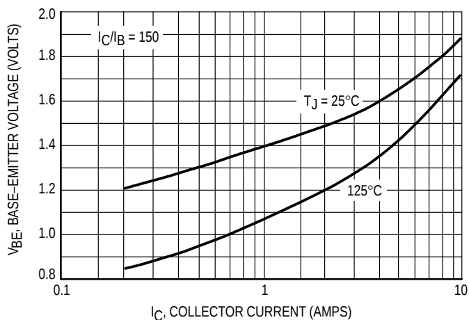
Figure 9. Base-Emitter Saturation Voltage
