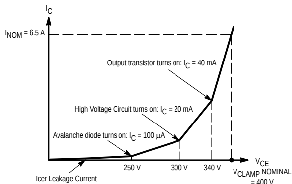
Figure 1. I_C = f(V_{CE}) Curve Shape
