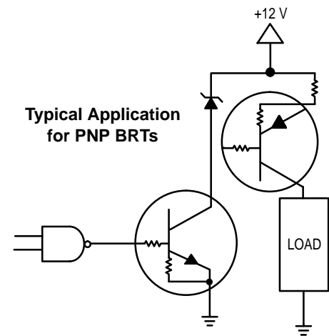
Figure 6. Inexpensive, Unregulated Current Source
