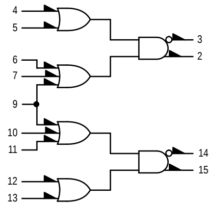
LOGIC DIAGRAM
