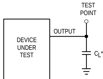
Figure 7. Test Circuit
