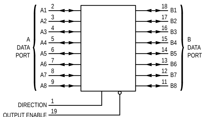
LOGIC DIAGRAM
