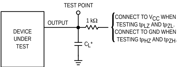
Figure 4. Test Circuit
