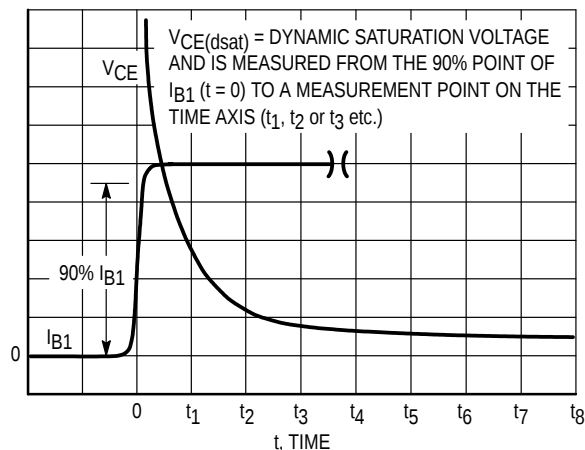
Figure 11. Definition of Dynamic Saturation Measurement
