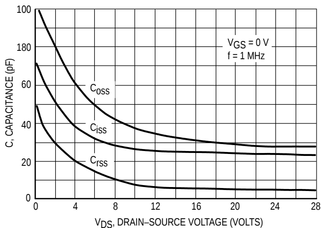
Figure 13. Capacitance versus Drain-Source Voltage* MRF136/MRF136Y
