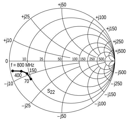
Figure 27. S_{22} , Output Reflection Coefficient versus Frequency V_{DS} = 28\text{ V} I_D = 0.5\text{ A}
