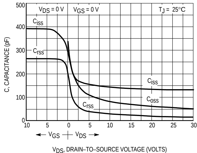
Figure 9. Capacitance Variation
