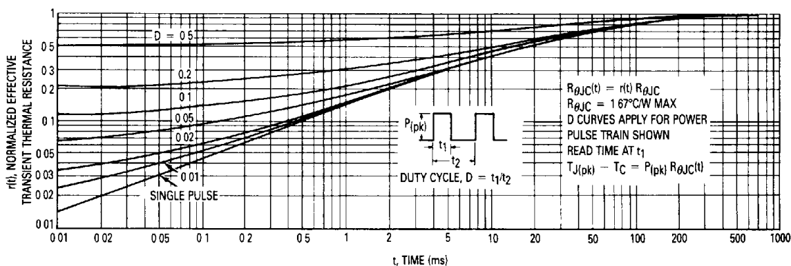
Figure 10. Thermal Response
