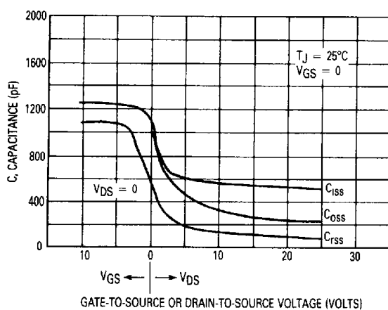
Figure 11. Capacitance Variation
