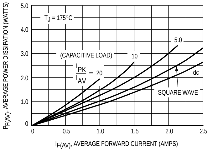
Figure 9. Power Dissipation
