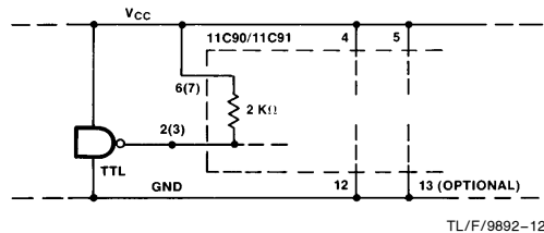
FIGURE 5. Using Internal Pull-Up with TTL Source
