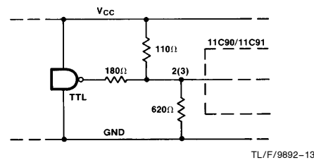
FIGURE 6. Faster Low Impedance TTL to ECL Interface
