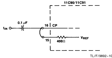
FIGURE 3. Capacitively Coupled Clocking
