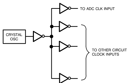
FIGURE 8. Isolating the ADC clock from digital circuitry
