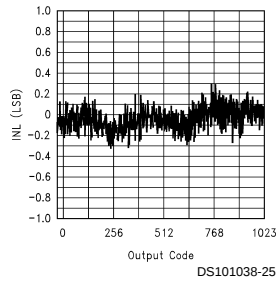
Typical INL
