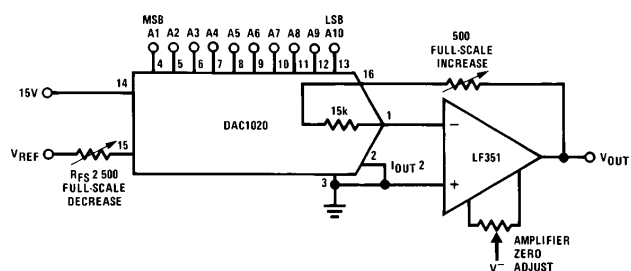
FIGURE 4. Full-Scale Adjust
