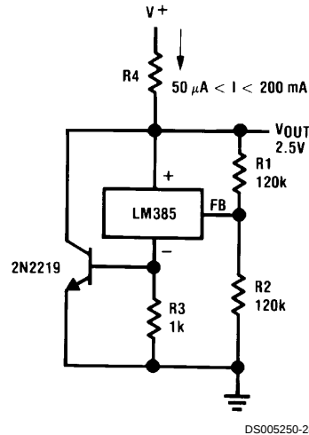
200 mA Shunt Regulator
