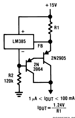
Current Source
