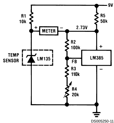
Centigrade Thermometer, 10mV/°C
