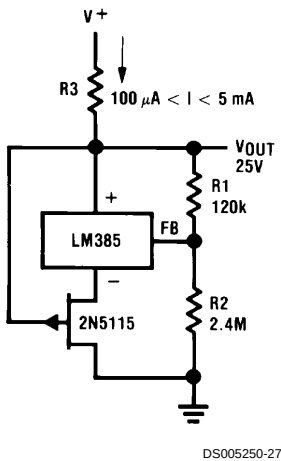
25V Low Current Shunt Regulator
