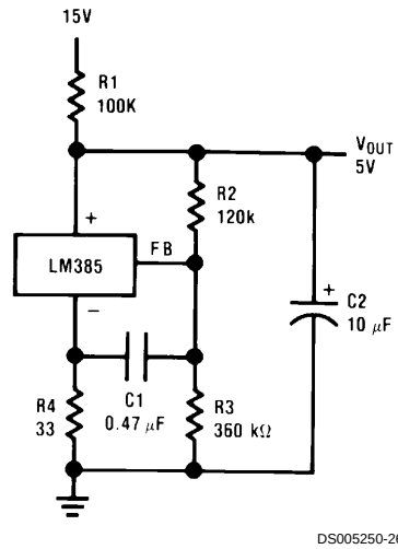
Low AC Noise Reference
