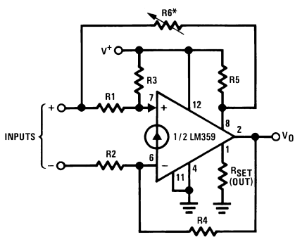
Difference Amplifier
