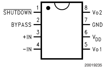
Top View Order Number LM4890M See NS Package Number M08A
