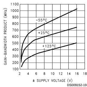
Gain-Bandwidth Product
